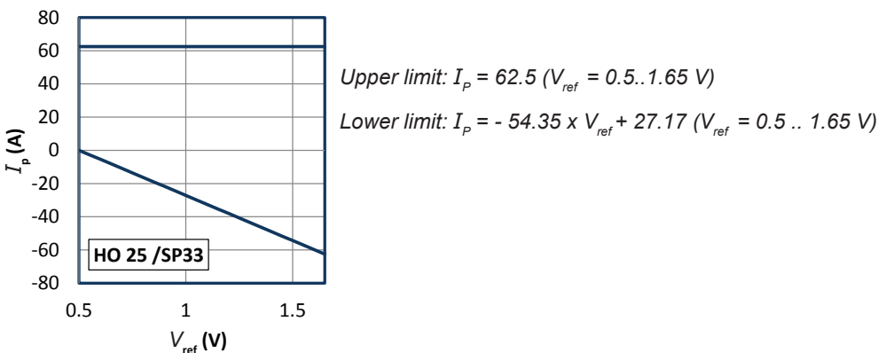
Figure 17 I_p vs V_{ref} for HO-NSM/SP33 series
