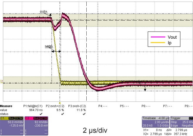
Figure 13: Step response
