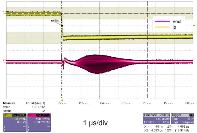
Figure 4: dv/dt
