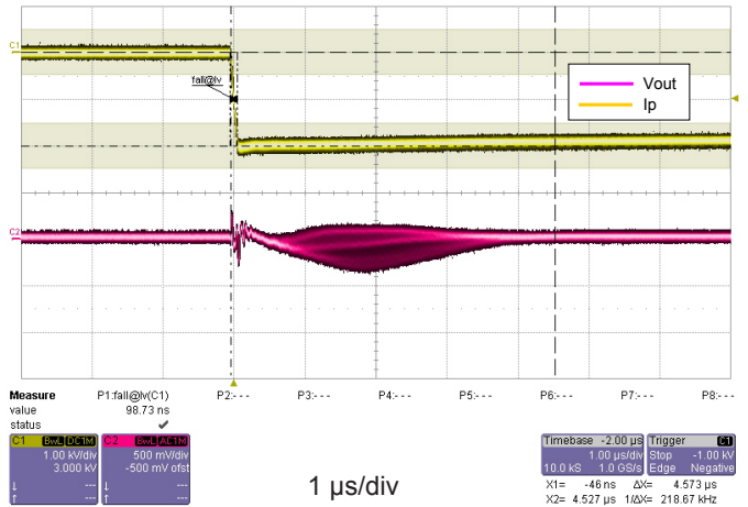
Figure 14: dv/dt
