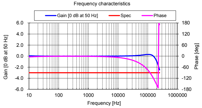
Figure 2: Frequency response
